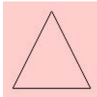
Figure 16.12. imagepolygon output.
