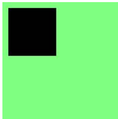
Figure 16.10. imagefilledrectangle output.
