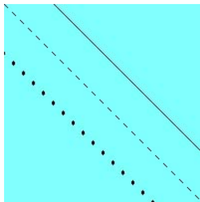
Figure 16.11. imageline output.
