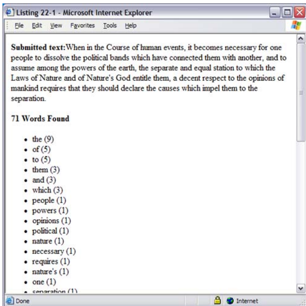
Figure 22.1. Output from Listing 22.1 .
