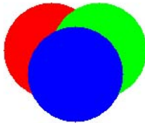
Figure 16.4. imagecolorallocate output.
