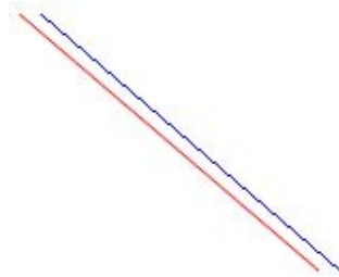
Figure 16.2. imageantialias output.
