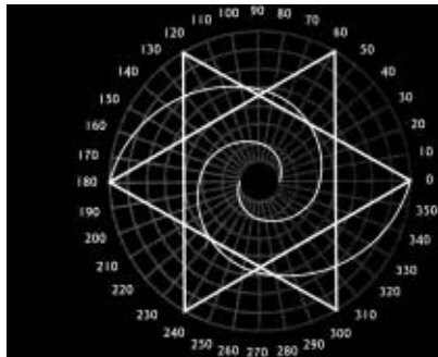
Fig. 8-31. Two spirals forming a star tetrahedron on a polar graph.
